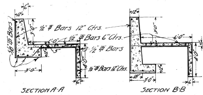
CONCRETE DROP Scale 1/4" = 1'-0"
