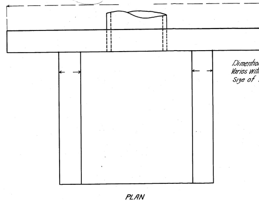
CONCRETE DROP Scale 1/4" = 1'-0"
