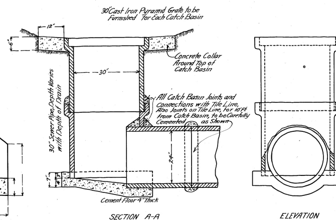
SPECIAL CATCH BASIN SCALE 3/4" = 1'
